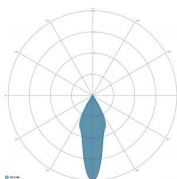
OPTICS: 4-ROTOSYMMETRICAL 30°
