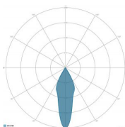
OPTICS: 4-ROTSYMMETRICAL 30°
