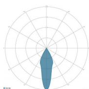
OPTICS: 4-ROTOSYMMETRICAL 30°
