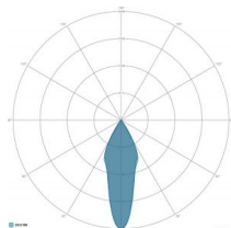
OPTICS: 4-ROTSYMMETRICAL 30°
