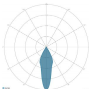
OPTICS: 4-ROTSYMMETRICAL 30°
