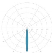
OPTICS: 6-ROSYMMETRICAL 10°
