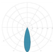
OPTICS: 5-ROTSYMMETRICAL 20°
