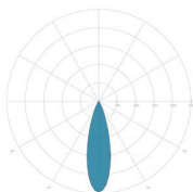
OPTICS: 5-ROTOSYMMETRICAL 20°
