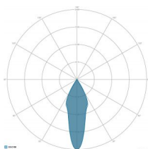
OPTICS: 4-ROSYMMETRICAL 30°
